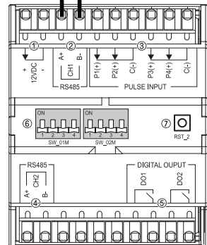
Meterinterface
