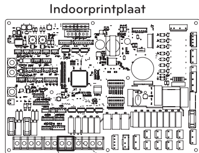
PUMP A2
