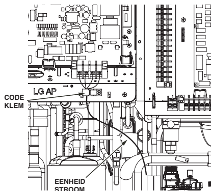
UN36A (5, 7, 9 kW)
